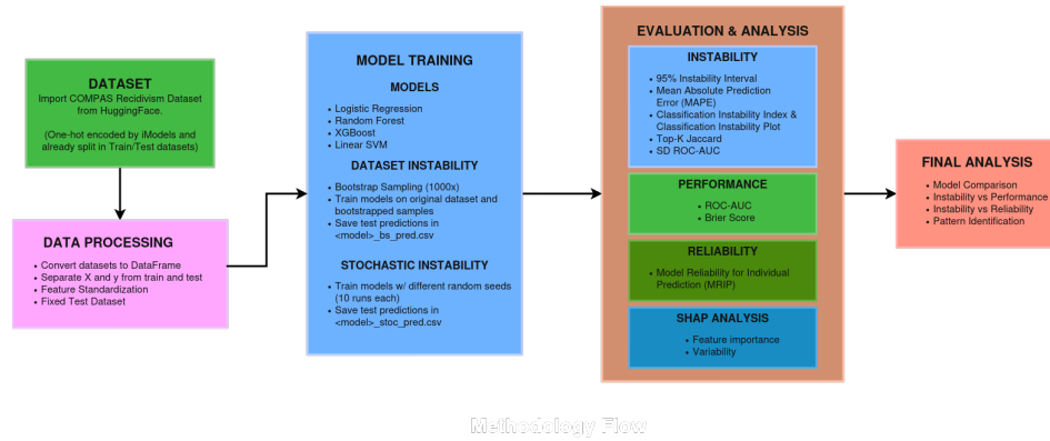
Figure 1: Overview of the proposed methodology for evaluating dataset and stochastic instability in machine learning models.
